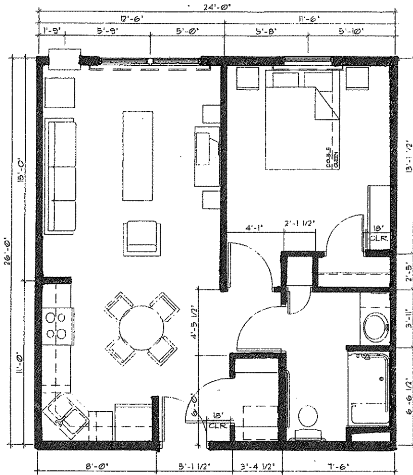
1 TYPICAL ONE BEDROOM UNIT A-4 SCALE: 1/4"=1'-0"
